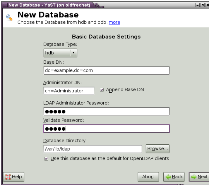
Figure 26.3 YaST LDAP Server—New Database
