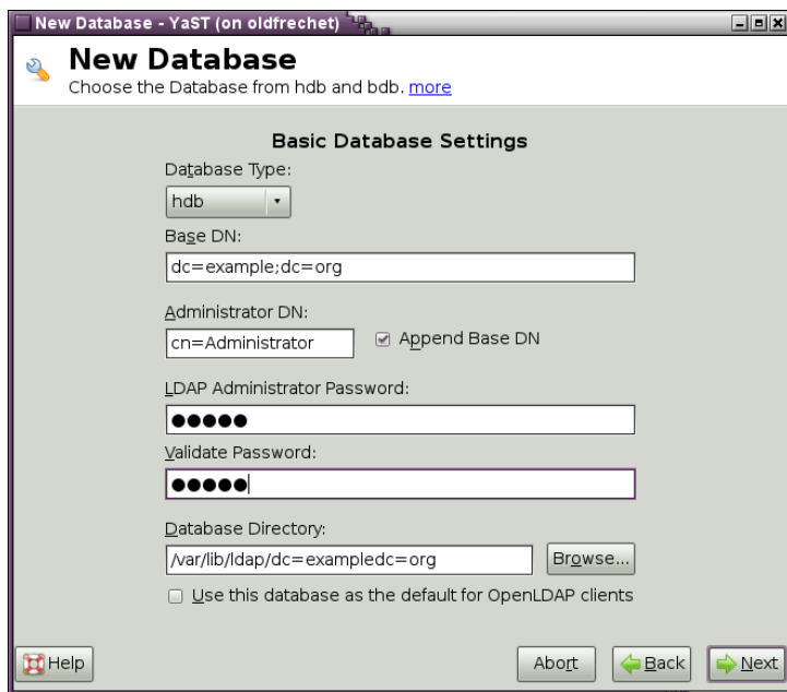
Figure 26.5 YaST LDAP Server Configuration
