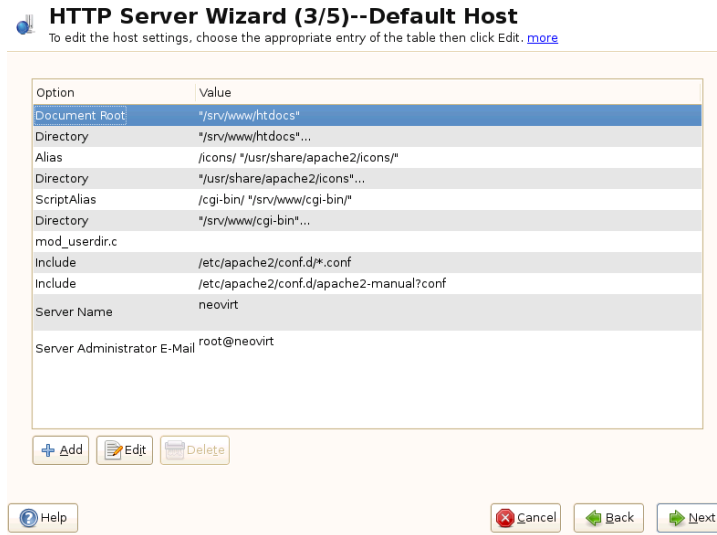
Figure 28.1 HTTP Server Wizard: Default Host
