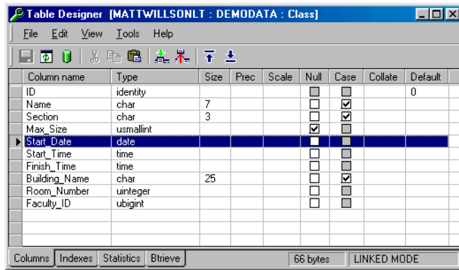
Figure 3-14 Table Designer
