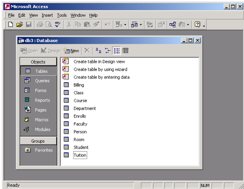
Figure 2-35 Using Pervasive Data in Microsoft Access
