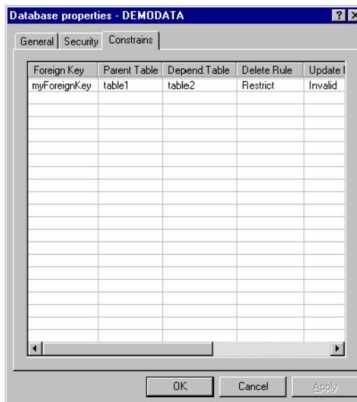
Figure 3-34 Database Properties
